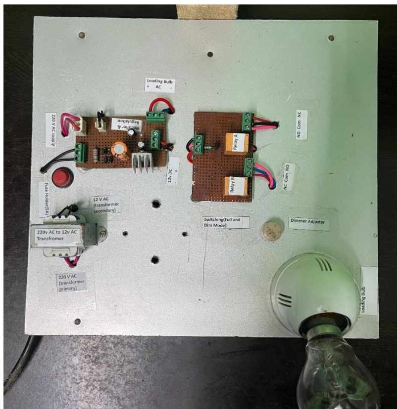
Fig 13: Top view of the developed model
